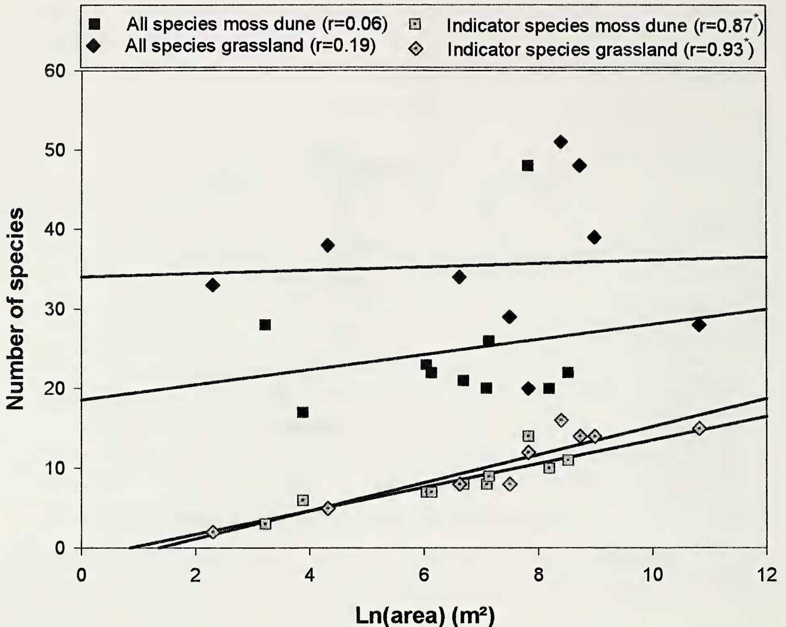
Figure 4.—Species-area relationship for all species and indicator species caught on moss dominated dry dunes and short grasslands from different sizes (Spearman correlation, *: P < 0.01 ).
